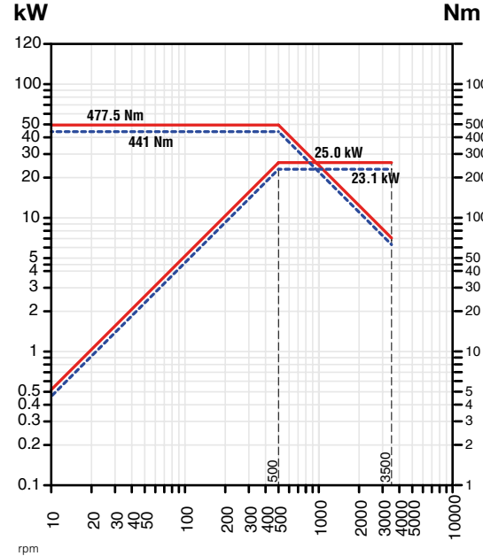
ASA 8 main spindle (80mm bar capacity)
